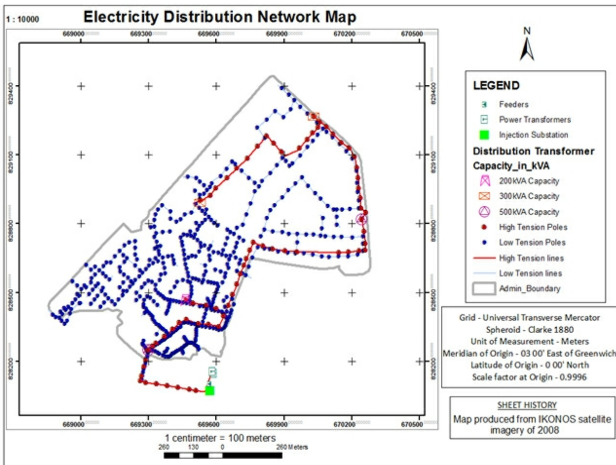
Fig 1: Electricity Distribution Network Map
