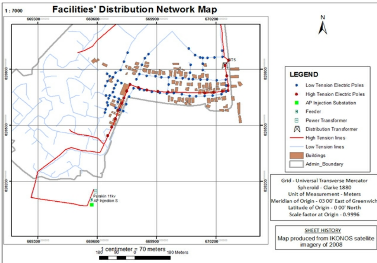
Fig. 2: Map showing the facilities involved in the distribution of electricity to consumers
