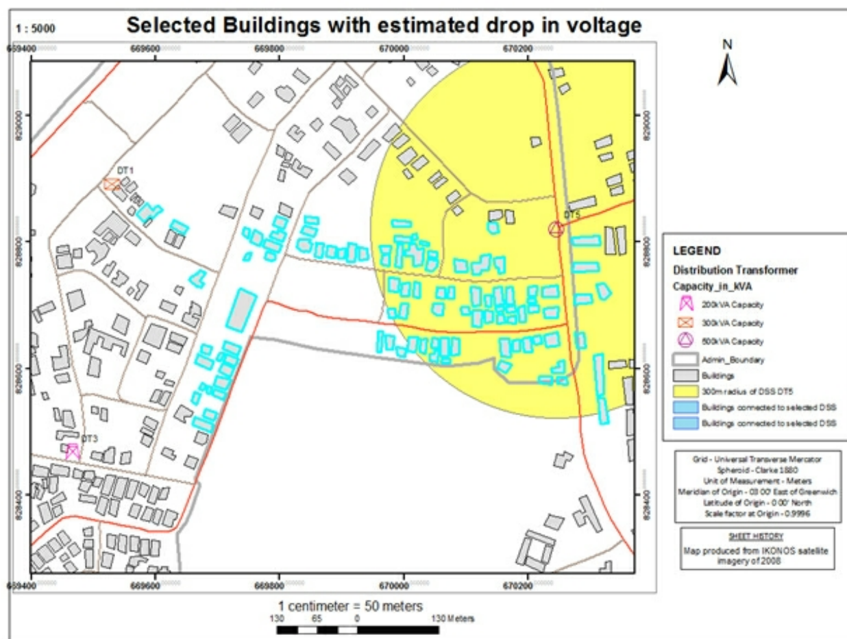
Fig 4: Selected Buildings with estimated drop in voltage
