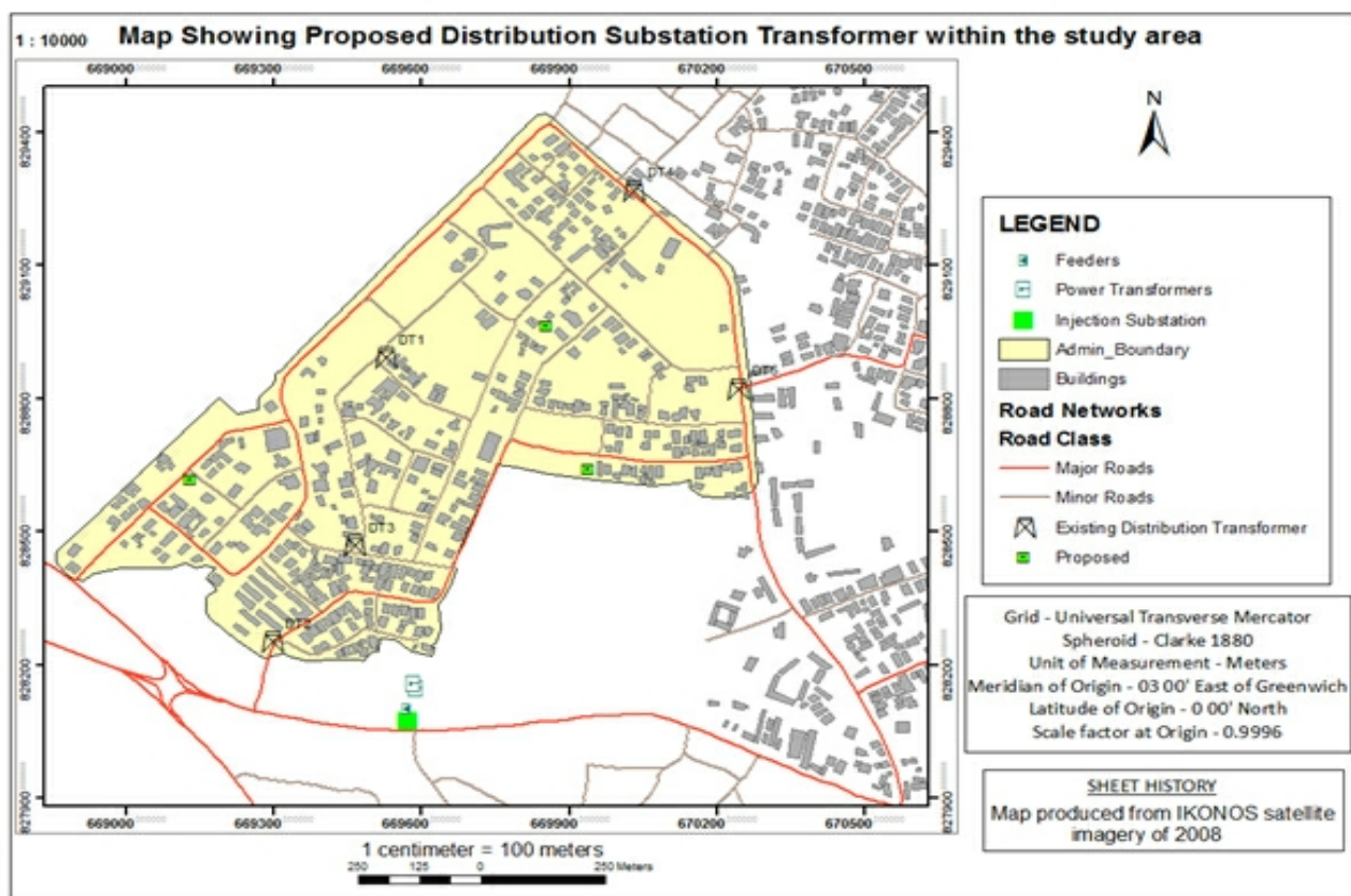
Fig 3: Map showing existing and proposed location of DSS
