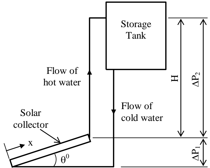
Fig. 1: The schematic diagram of natural circulation solar water heater.
