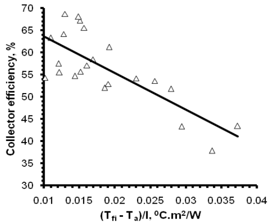
Fig. 6. Collector efficiency versus incident solar radiation.
