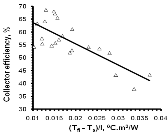
Fig. 4: Variation of the collector efficiency with performance coefficient (T_{fi} - T_a)/I .
