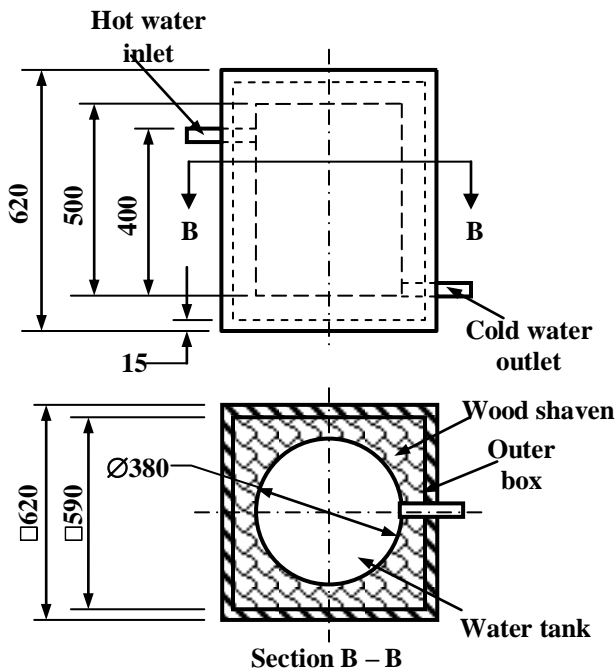
Fig. 3: Storage tank
