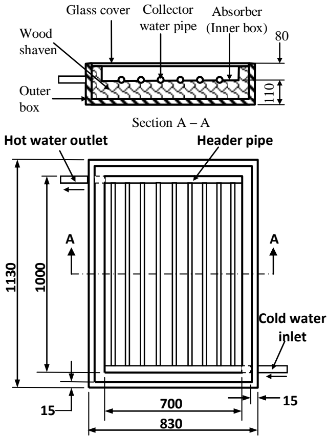
Fig. 2: Flat-plate solar collector with water pipes
