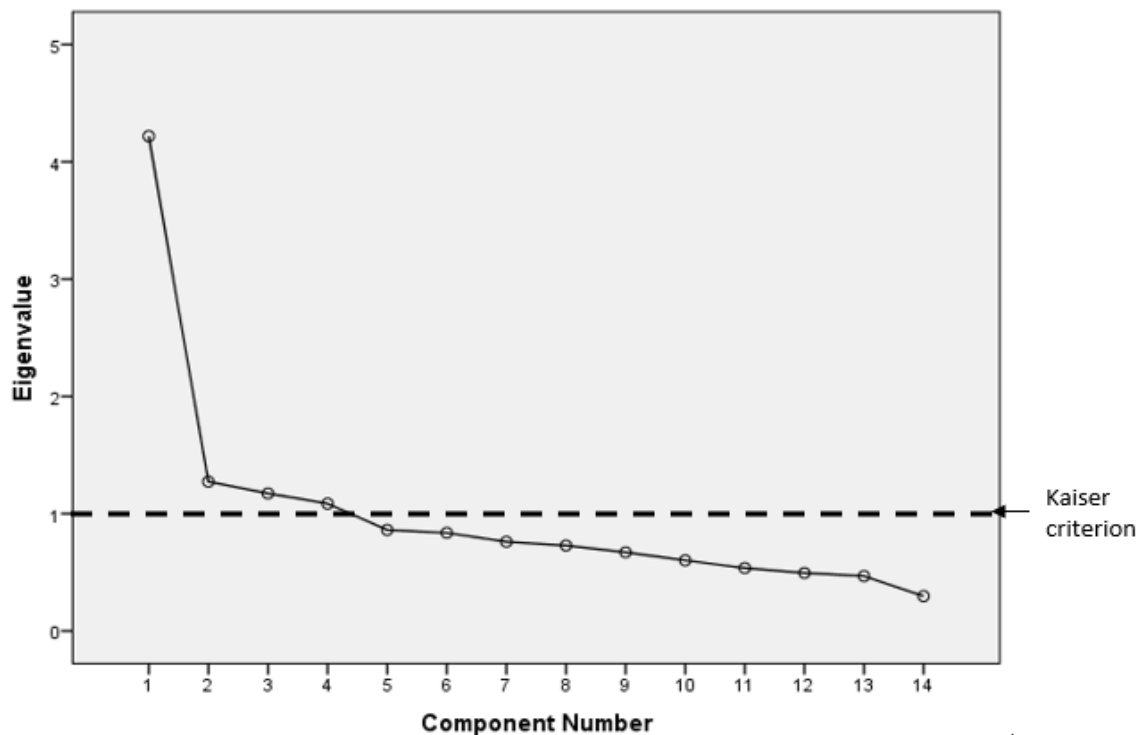
Figure 1: Scree Plot
