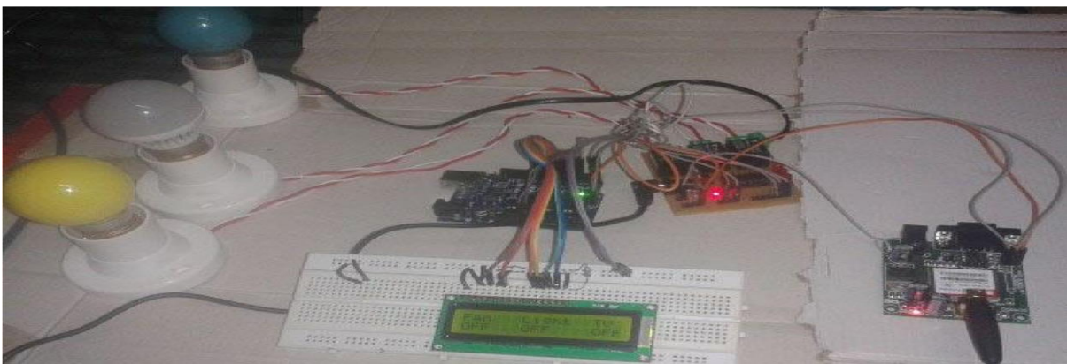
Fig. 24: design setups
