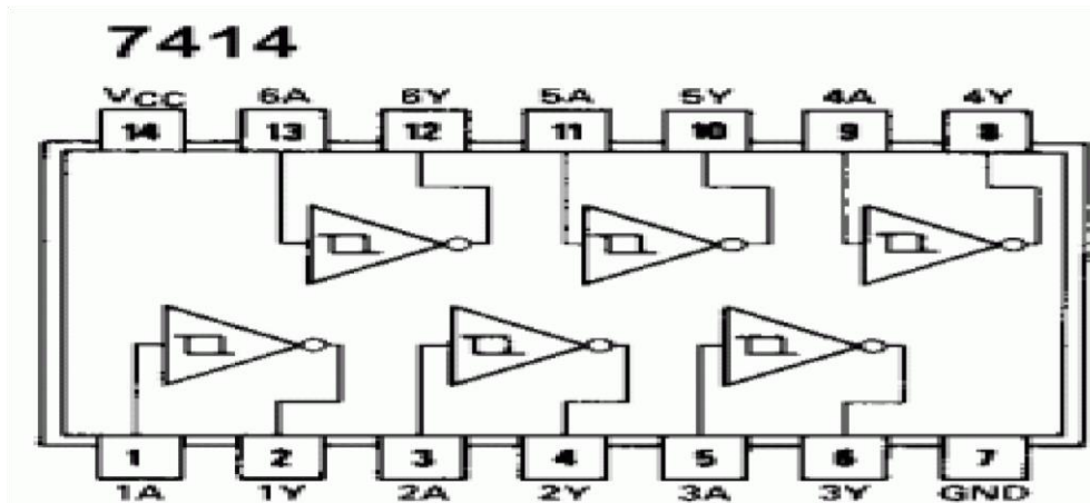
Fig. 7: CD7414
