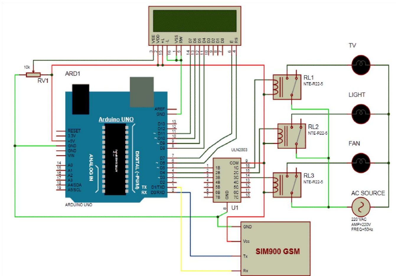
Fig 16 Circuit Diagram of the Project
