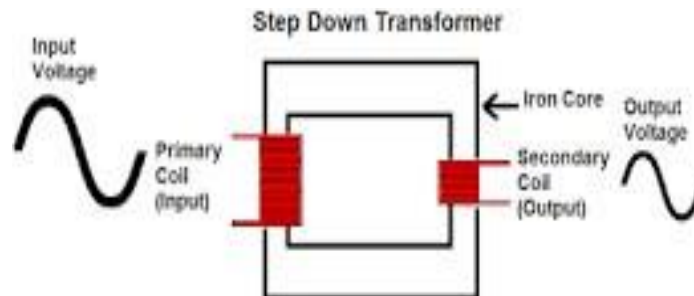
Fig.3: Transformer
