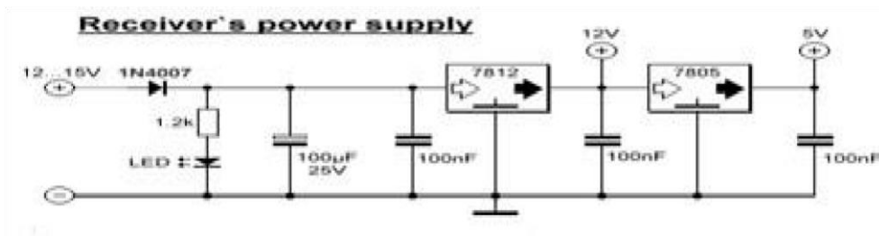
Fig: 18: The power supply or receiver
