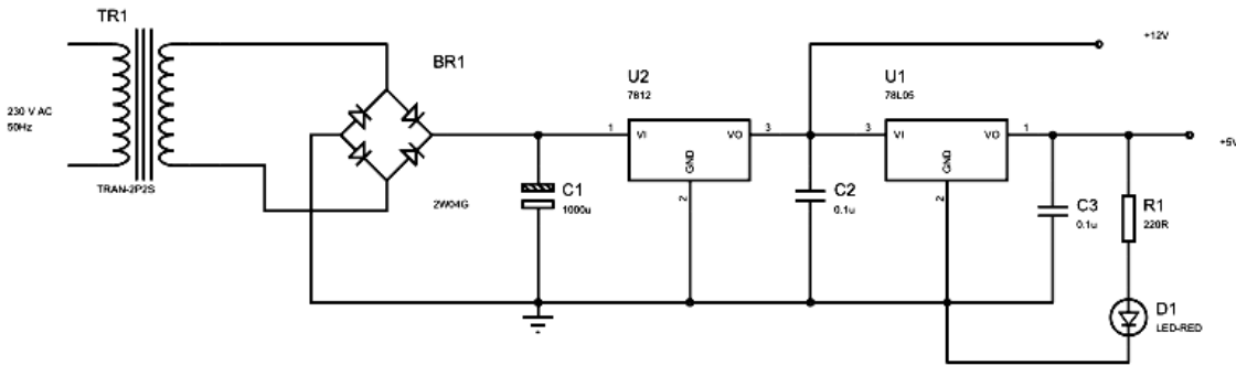
Fig 3.7 Power supply
