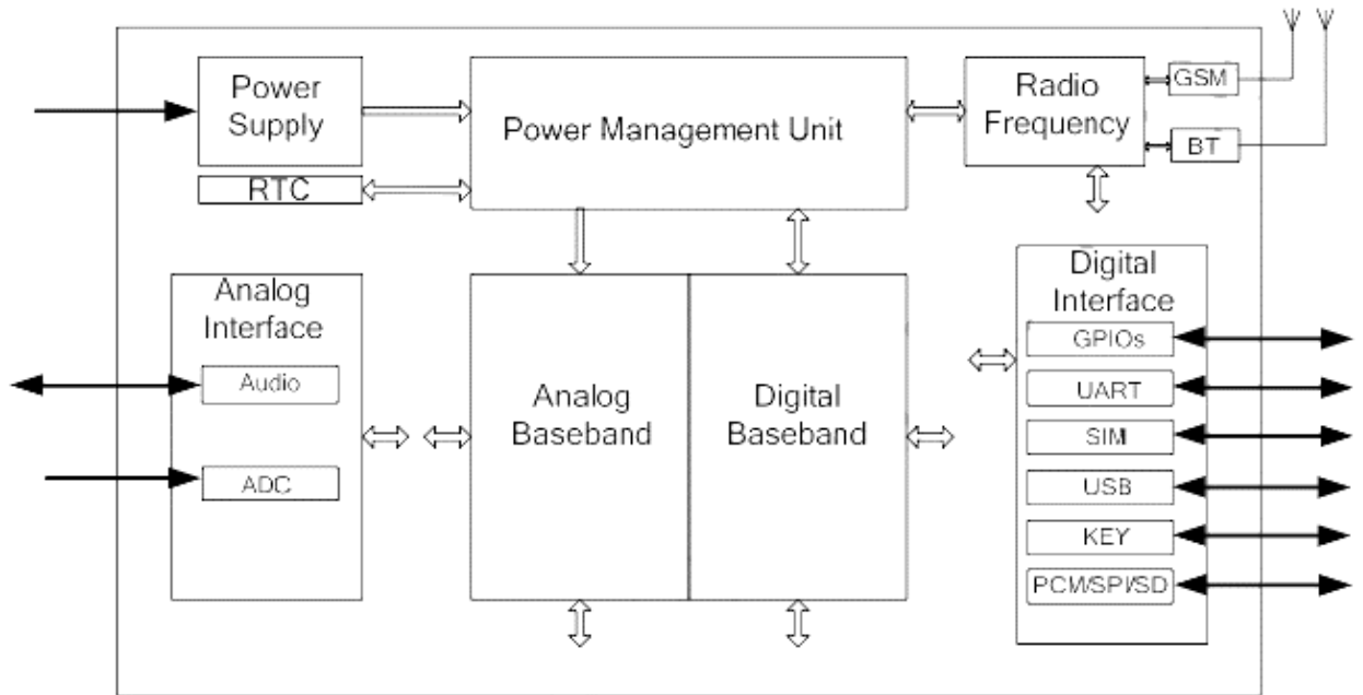
Fig. 3.6: SIM800 functional diagram (SIMCOM, 2015)
