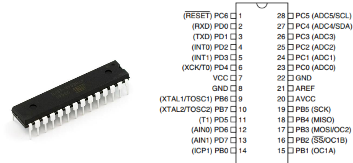
Fig. 3.2 pin diagram of microcontroller ATMEGA 8 (Atmel, 2013)
