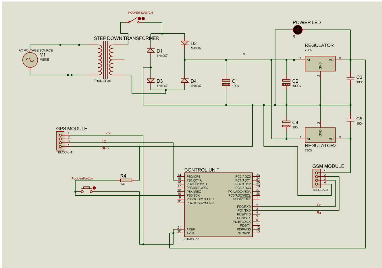
Fig. 3.9: complete Circuit Diagram of VAAT system
