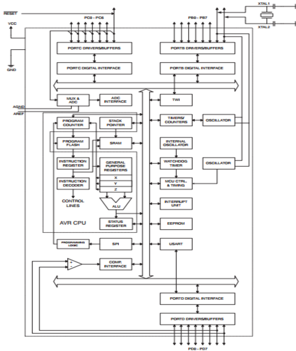
Fig 3.2 Block Diagram ATMEGA 8 (Atmel, 2013)
