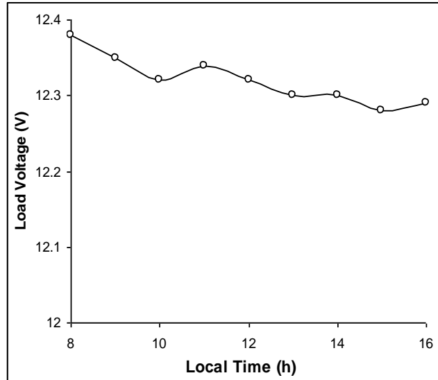
Fig. 8. Diurnal variation of battery output during the office hours.
