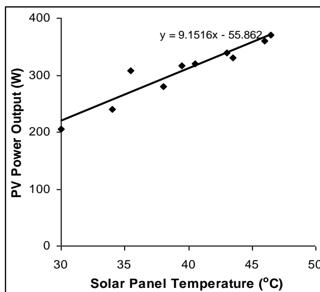
Fig. 11. Variation of PV power output with the solar panel temperature.
