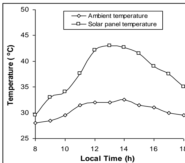
Fig. 7. A typical day results of variation of ambient and solar panel temperatures 3 rd September, 2008.
