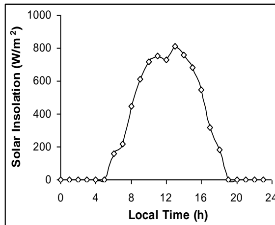
Fig. 9. A typical day results of the variation of solar insolation on the 1st of September, 2008.
