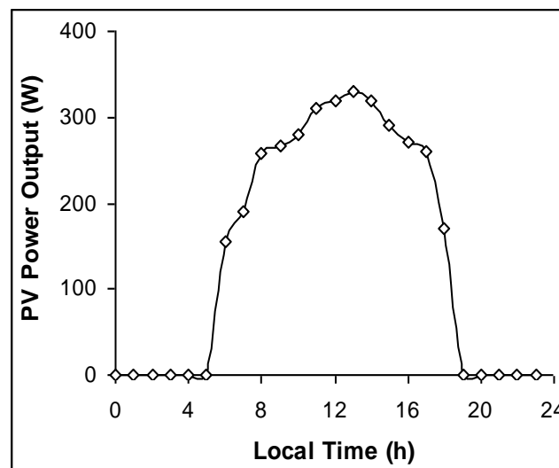
Fig. 10. A typical day hourly results of photovoltaic power output.
