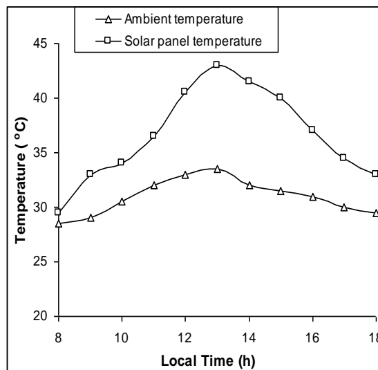
Fig. 6. A typical day results of variation of ambient and solar panel temperatures for 1 st September, 2008.
