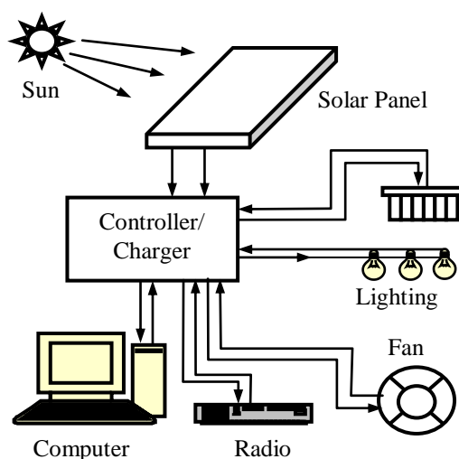
Fig. 2. Schematic of the PV- System for Electrification
