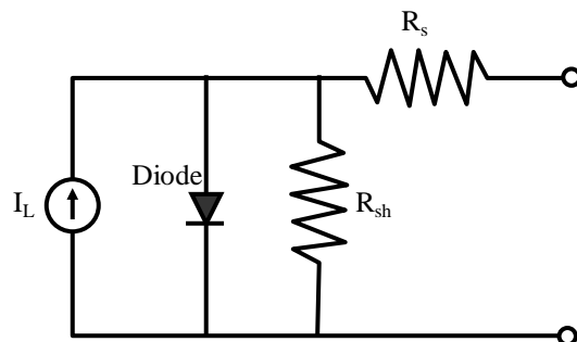
Fig. 1. Equivalent circuit of a solar cell [10].
