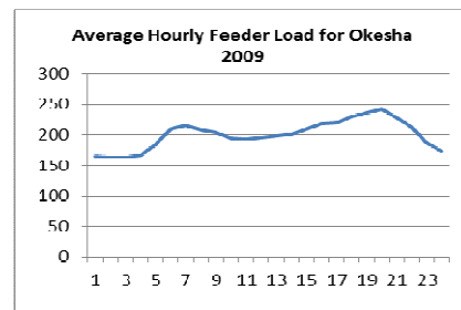
Figure 9. Average Hourly Feeder Load Curve for Okesha, 2009.
