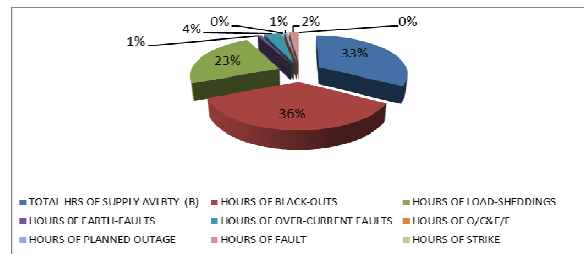
Figure 13. parameters on Ajilosun Feeder, 2009.
